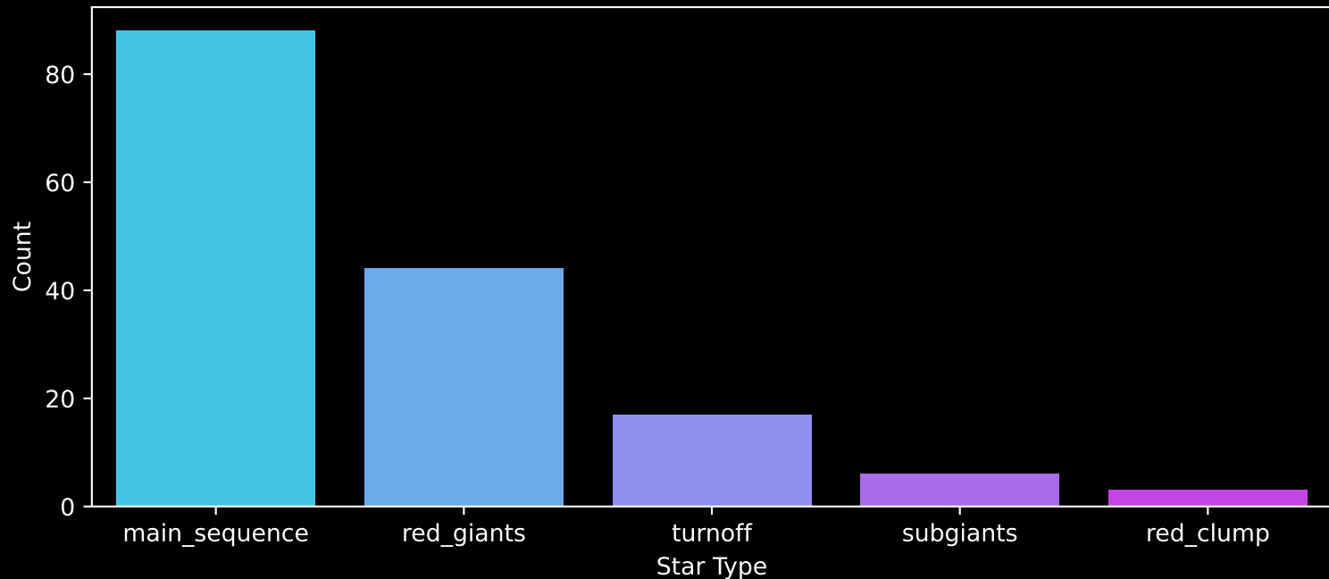
APOGEE DR17 Field: [SCULPTOR] Count plot of Star Type
