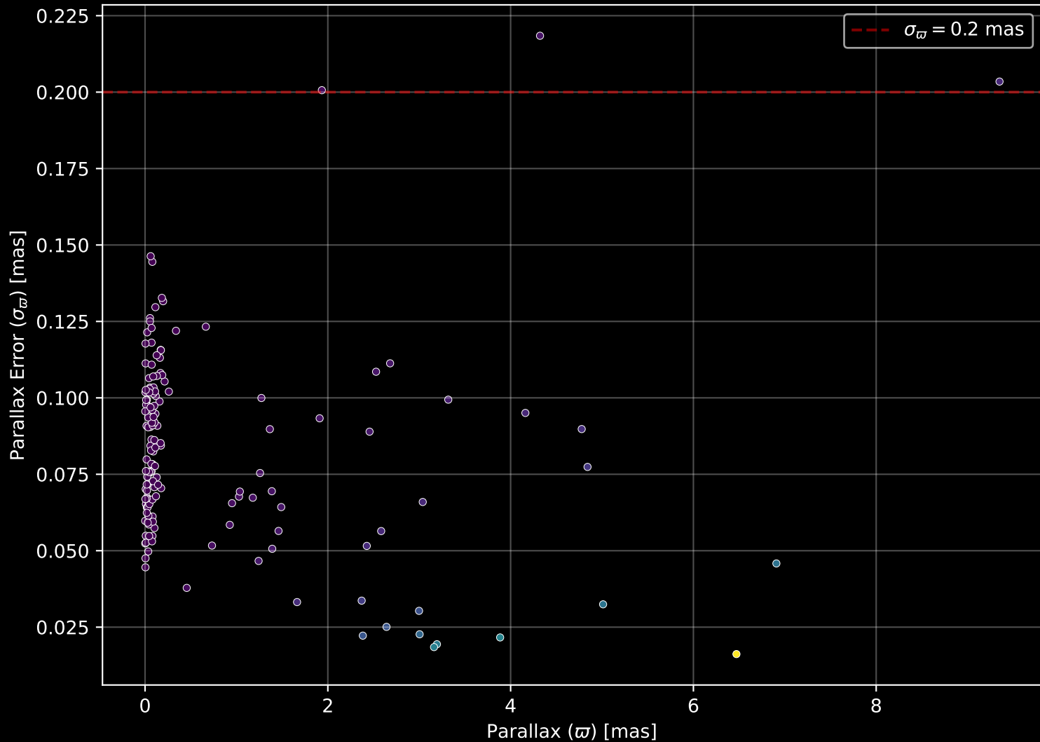
APOGEE DR17 Field: [SCULPTOR] Parallax Quality (n= 158)
