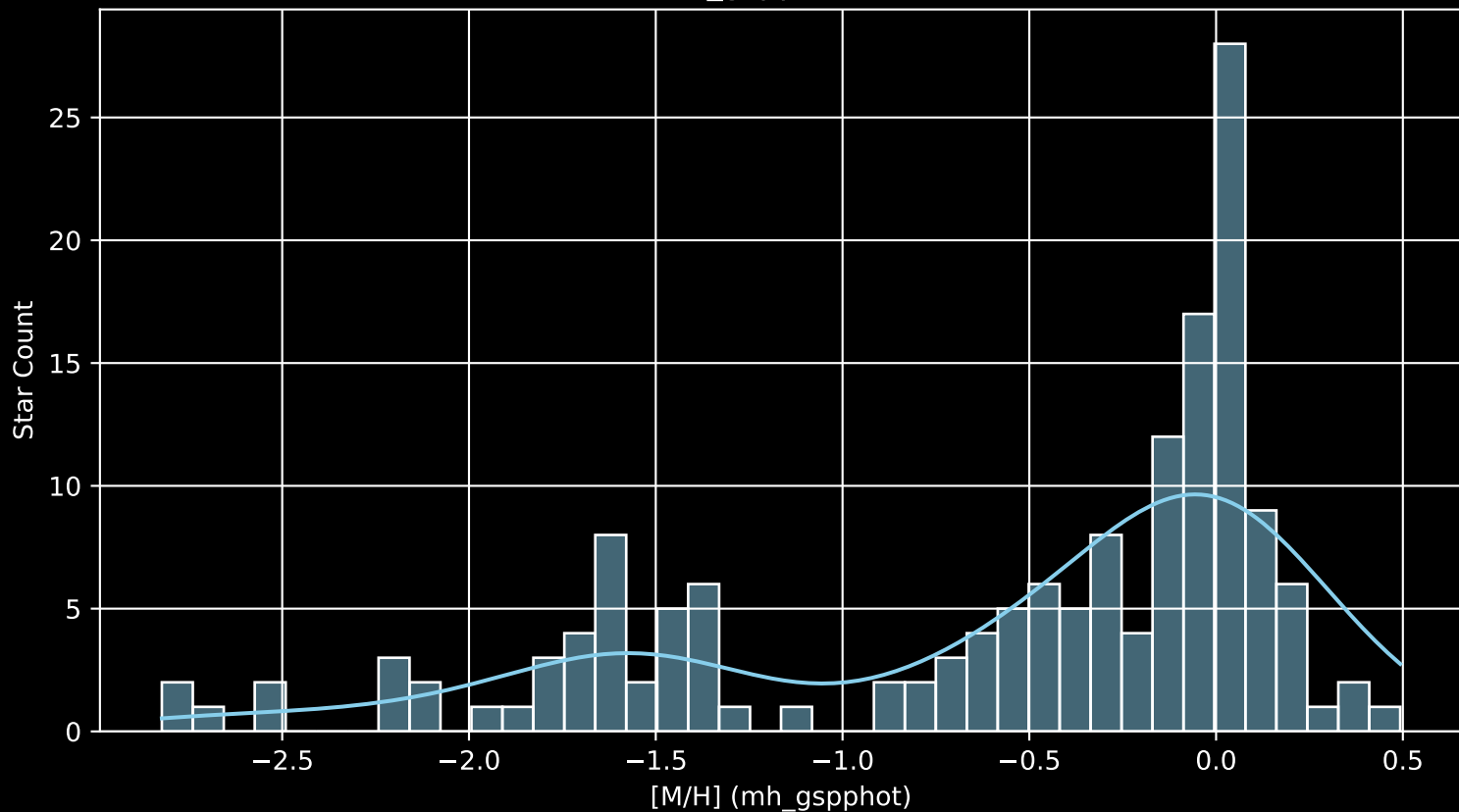
APOGEE DR17 Field: [SCULPTOR [M/H] (mh_gspphot) (n= 157)
