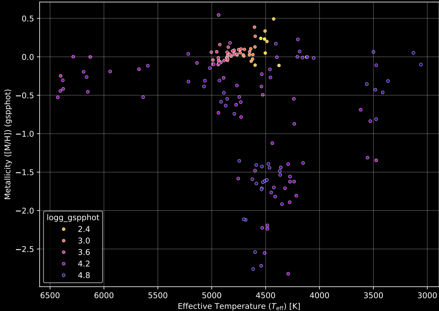
APOGEE DR17 Field: [SCULPTOR] Stellar Population Parameters (n= 158)
