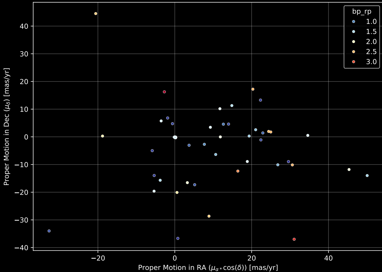
APOGEE DR17 Field: [SCULPTOR] Proper Motion Diagram (n= 158)
