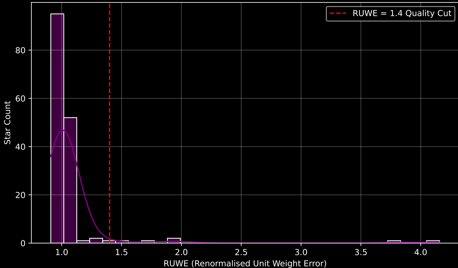
GAPOGEE DR17 Field [SCULPTOR] RUWE Distribution (n= 157)
